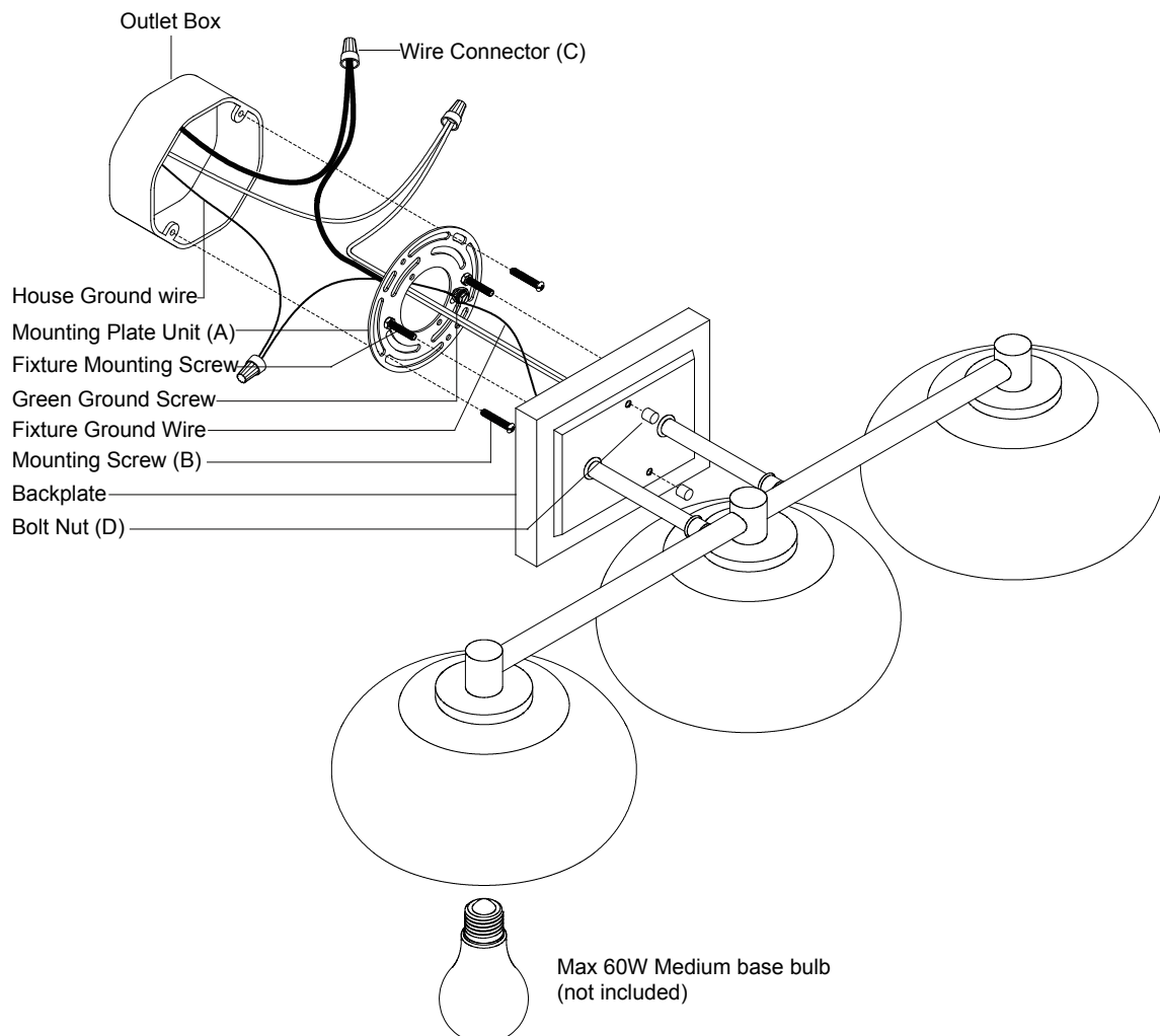
Mounting Plate Unit (A)
